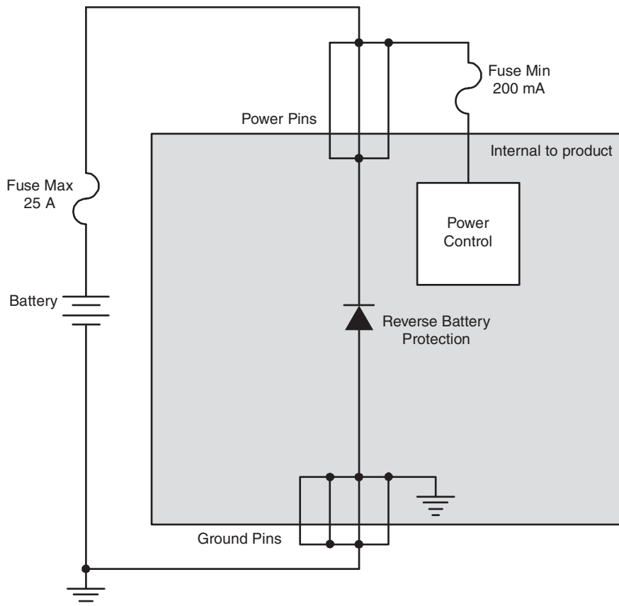
Figure 13: Logic and output power installation connections
