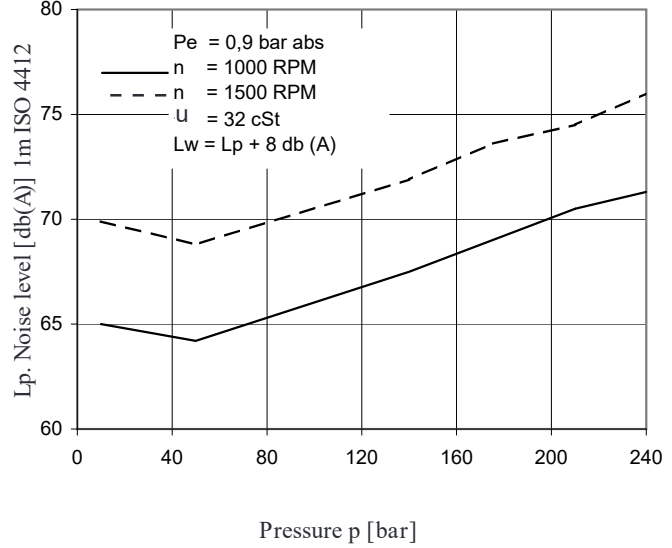
NOISE LEVEL (TYPICAL) - T7DDB - B31 - B31 - B10
