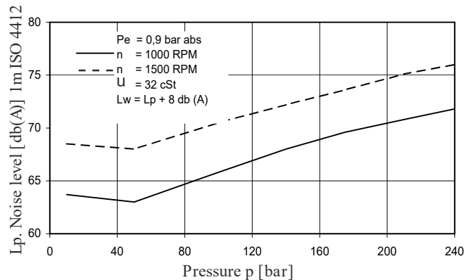
NOISE LEVEL (TYPICAL) - T7DDS - B31 - B31
