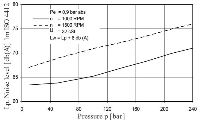
NOISE LEVEL (TYPICAL) - T67EC - 050 - B22
