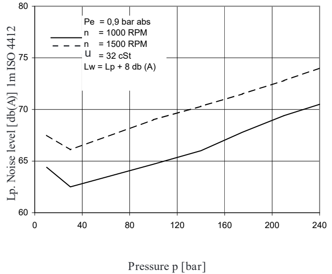
NOISE LEVEL (TYPICAL) - T7DCB - B38 - B22 - B10
