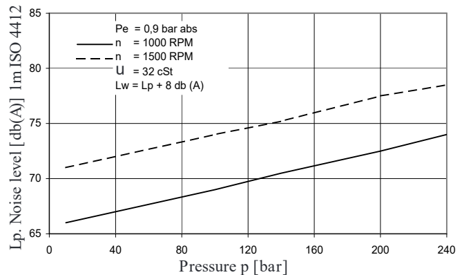
NOISE LEVEL (TYPICAL) - T7EE - 050 - 050
