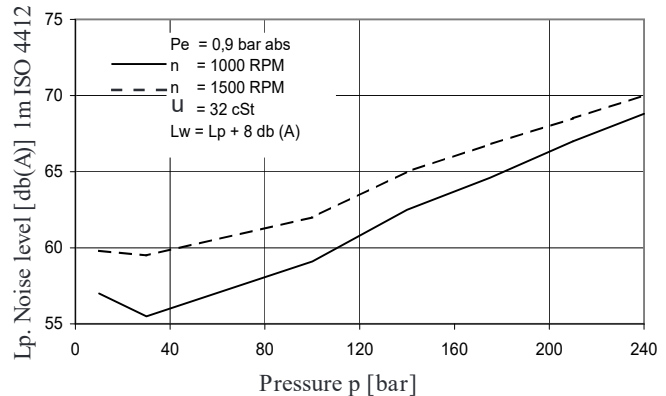
NOISE LEVEL (TYPICAL) - T67CB - B14 - B03
