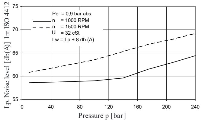
NOISE LEVEL (TYPICAL) - T6C - B22
