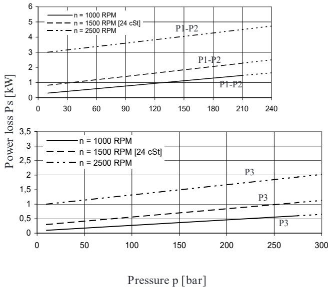
POWER LOSS HYDROMECHANICAL (TYPICAL)
