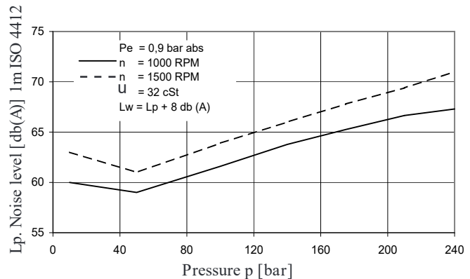
NOISE LEVEL (TYPICAL) - T7DBS - B31 - B10
