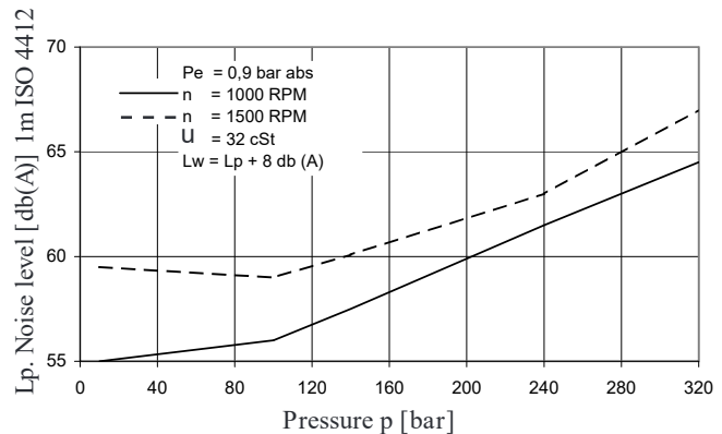
NOISE LEVEL (TYPICAL) - T7BB - B10 - B04
