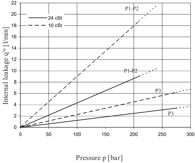
INTERNAL LEAKAGE (TYPICAL)
