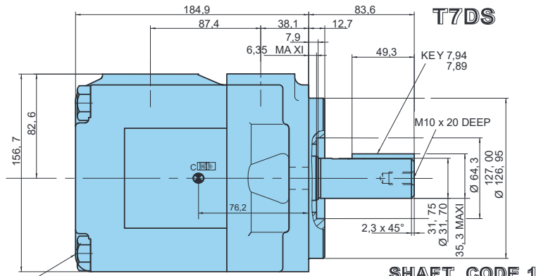
SHAFT CODE 1 (Keyed SAE C)
