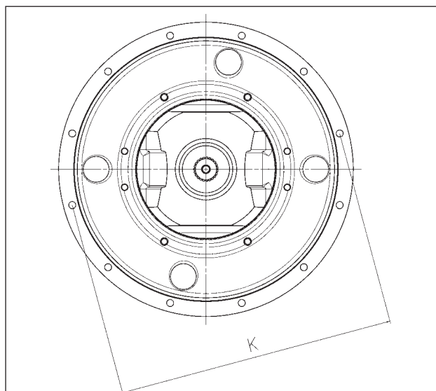
SAE bell housing
