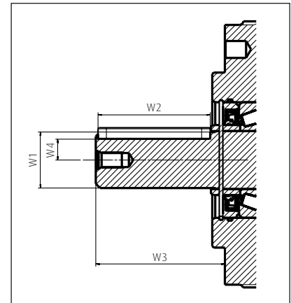
Mounting flange
