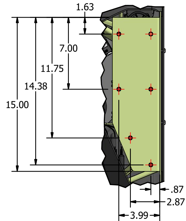
DETAIL A SCALE 3:16
