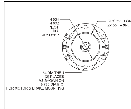
"B" Option SAE 'B' 2 Bolt Thru
