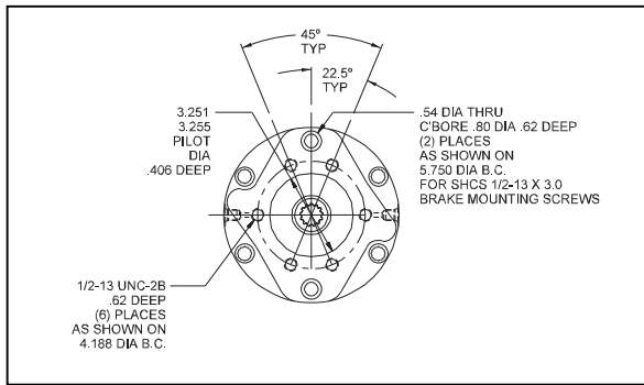
"A" Option SAE 'A' 2 & Modified 4 Bolt
