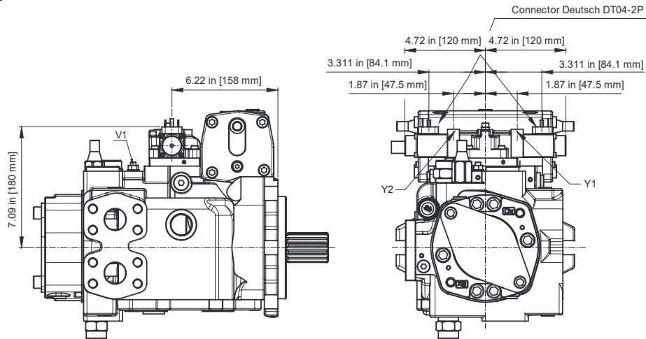
Y1-Y2: Control piloting pressure ports – 1/4" (BSPP) V1: Adjustable throttle valve
