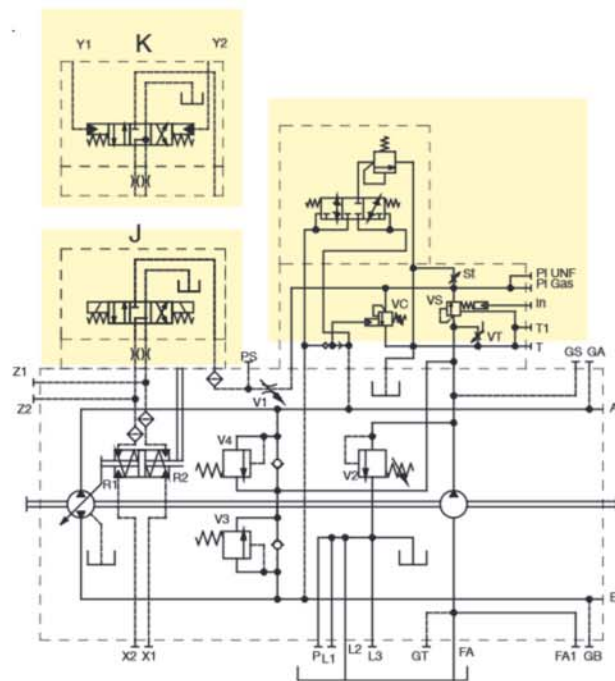
C081 Electric (J) / Hydraulic (K) Automotive With Hydraulic Inching + Flushing Valve
