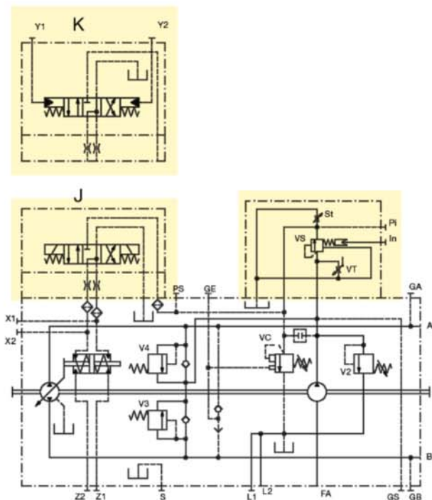
C055 Electric (J) / Hydraulic (K) Automotive With Hydraulic Inching + Flushing Valve
